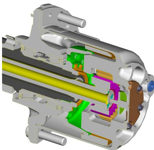
Current Hollow Shaft Design
