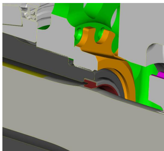
New Axial Breathing Seal and Solid Shaft
