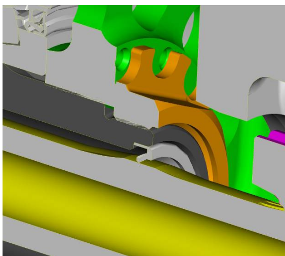
Current Axial Lip Seal and Hollow Shafts
